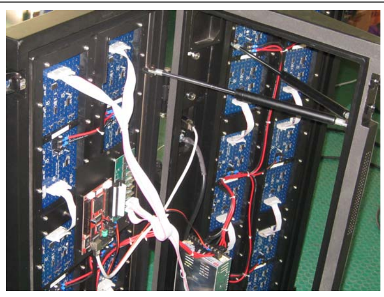
This is prop up structure
